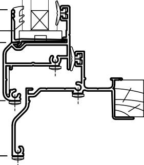
DETAIL E-E
